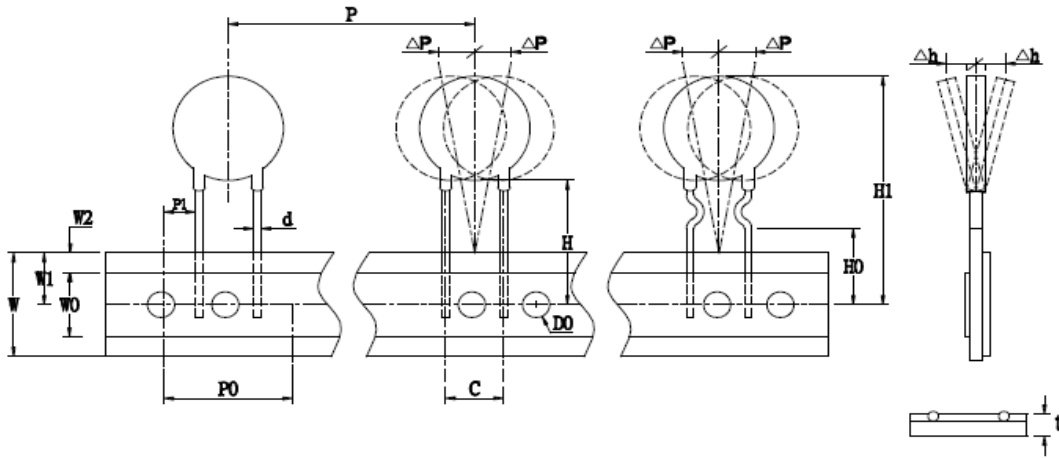
Fig.7 For KRG0600250-KRG0600375
