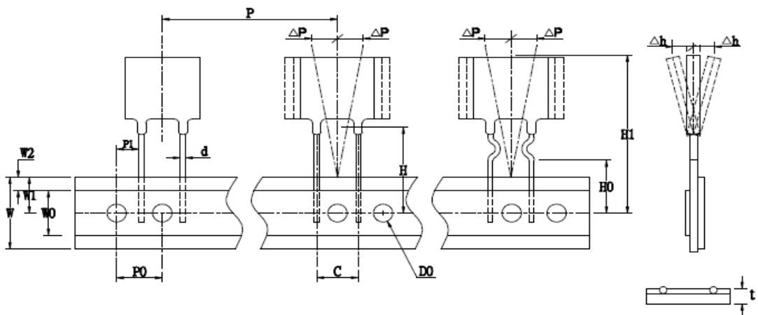
Fig.6 For KRG0600010-KRG0600185
