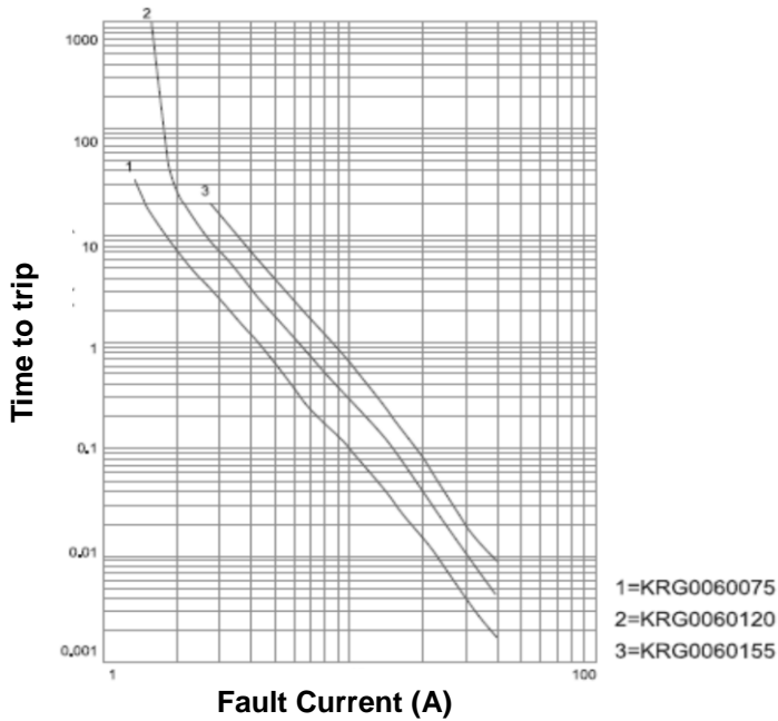
KRG006 Series
