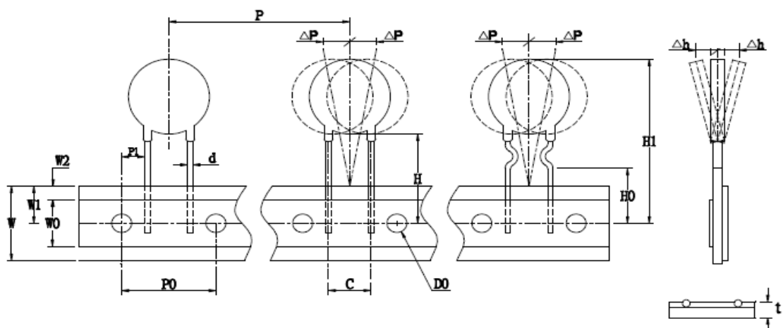
Fig.6 For KRG0600010-KRG0600185
